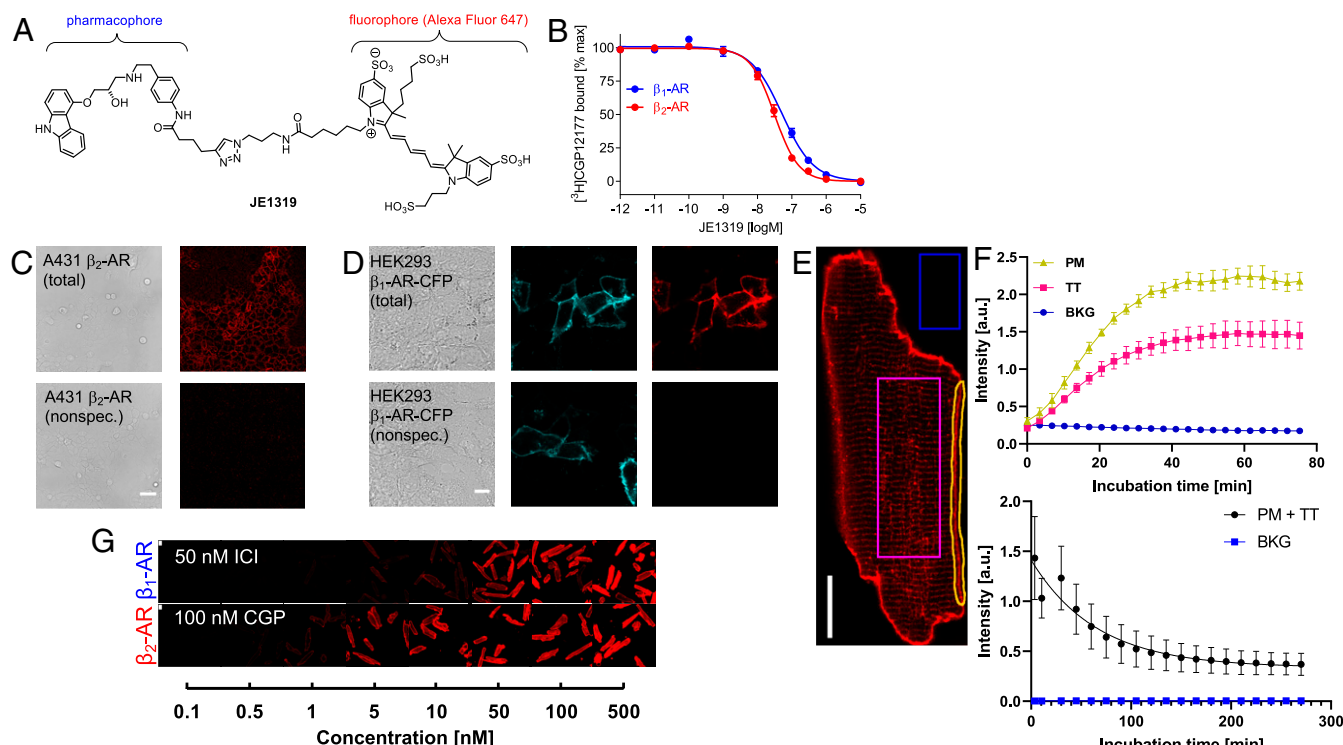
Fig. 1. Labeling of \beta -ARs in live cells with the ligand JE1319. ( A ) Chemical structure of the fluorescent ligand JE1319, a carazolol-Alexa647 conjugate. ( B ) Radioligand binding displacement experiments performed on intact HEK293T cells overexpressing either the \beta_1 -AR (blue dots) or the \beta_2 -AR (red dots), yielding K_i values of 42 \pm 8 nM ( n = 2 transfections) and 22 \pm 3 nM ( n = 8 transfections) for \beta_1 - and \beta_2 -AR, respectively. Error is SEM. ( C ) Endogenous \beta_2 -ARs were stained with 5 nM JE1319 in A431 cells (Upper); nonspecific binding was determined upon displacement with 50 nM ICI 118,551 (Lower). (Scale bar: 50 \mu\text{m} [ n = 2 imaging sessions].) ( D ) HEK293AD cells were transfected with \beta_1 -AR-CFP and stained with 5 nM JE1319 (Upper); nonspecific binding was determined in the presence of 100 nM CGP 20712 (Lower). (Scale bar: 10 \mu\text{m} [ n = 3 transfections].) ( E ) Image of a CM stained with 5 nM JE1319. Three regions of interest (ROIs) each were drawn on the membrane (PM), the inside of the cell (TT), and in the background (BKG). (Scale bar: 20 \mu\text{m} [representative of n = 3 CM preparations].) ( F , Upper) Time course of ligand binding from the three ROIs, such as those highlighted in E and ( F , Lower) time course of ligand dissociation in \beta_2 -AR-TG32 CMs. Errors are SD. a.u., arbitrary units. ( G ) Ligand binding series with different concentrations of JE1319 on adult CMs isolated from \beta_1 -AR-TG4 and \beta_2 -AR-TG32 mice and cultured for 1 d with either 50 nM ICI118,551 or 100 nM CGP 20712. Image contrast used in G is lower with respect to the one used in E . (Scale bar: 20 \mu\text{m} .)
